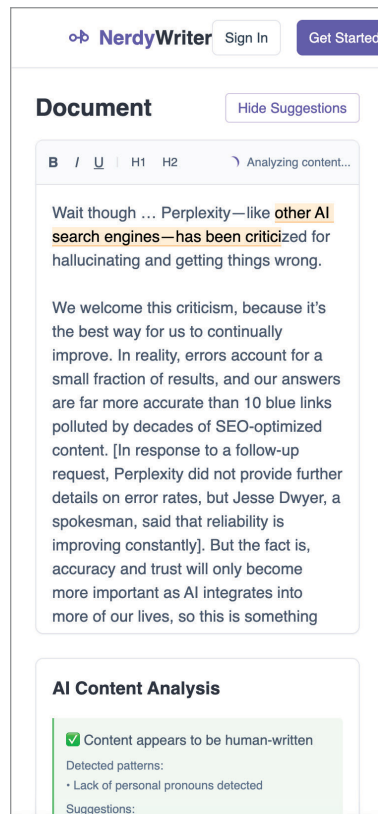
Figure 4 (above). An early prototype of NerdyWriter, a Grammarly-style writing tool built with Lovable.ai using “vibe coding” (Lovable, n.d.). Though AI models are not fully integrated, this mockup helps explore user flows and edge cases. The screenshot shows AI-generated content, inline grammar suggestions, and a scrollable horizontal layout for suggestion cards. It also raises critical UX questions: What if AI analysis fails? Can users regenerate or prompt AI? How do we distinguish between AI and user-edited or pasted content? This approach enables early thinking around product behavior and design, even before full AI integration.
