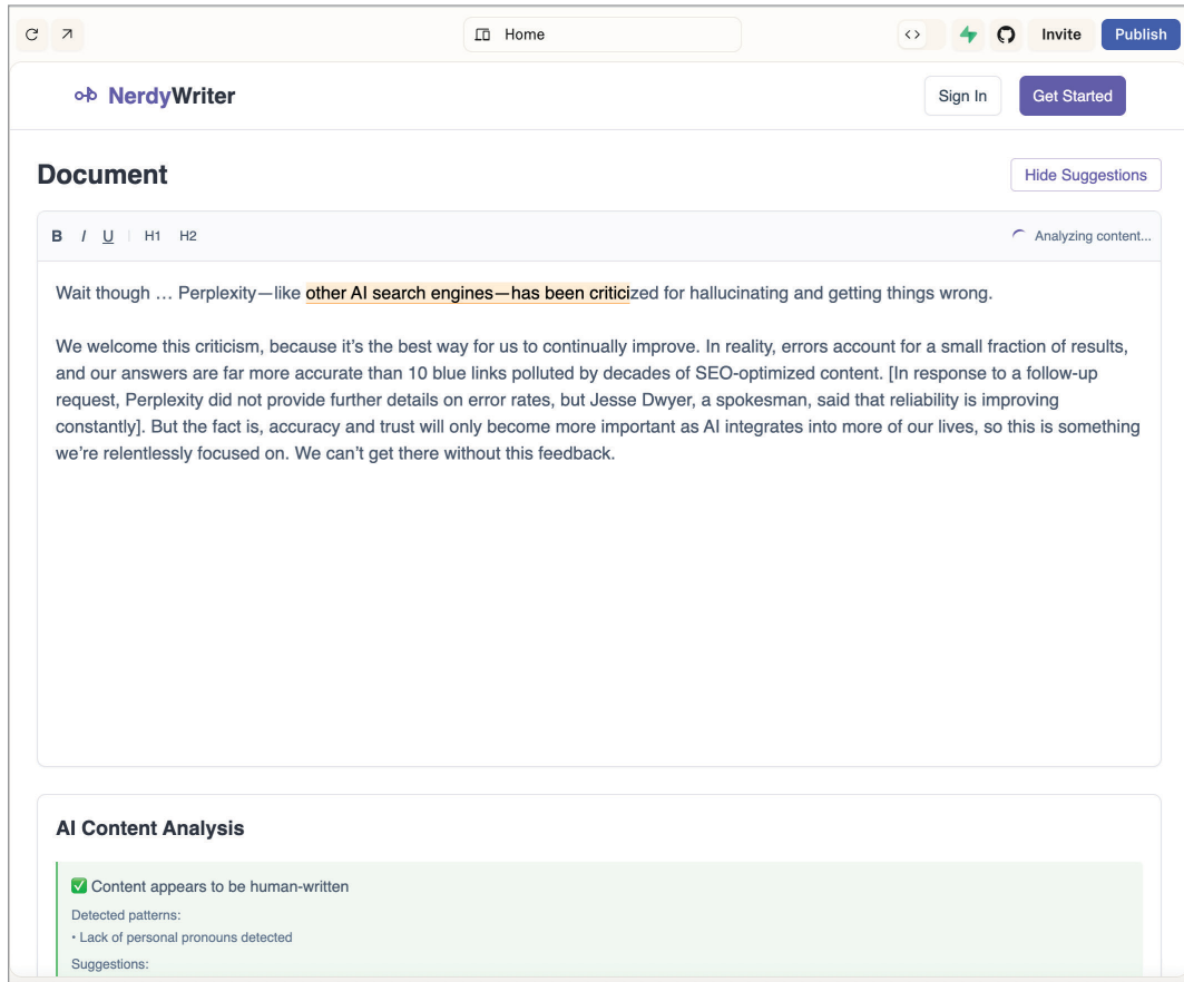
Figure 4 (above). An early prototype of NerdyWriter, a Grammarly-style writing tool built with Lovable.ai using “vibe coding” (Lovable, n.d.). Though AI models are not fully integrated, this mockup helps explore user flows and edge cases. The screenshot shows AI-generated content, inline grammar suggestions, and a scrollable horizontal layout for suggestion cards. It also raises critical UX questions: What if AI analysis fails? Can users regenerate or prompt AI? How do we distinguish between AI and user-edited or pasted content? This approach enables early thinking around product behavior and design, even before full AI integration.
